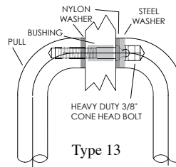
Type 13 Glass Door Back to Back Mount
