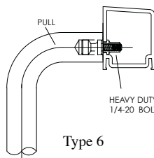
Type 6 Fully Concealed Mount
