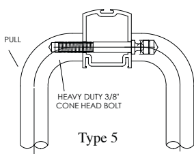
Type 5 Back to Back Mount
