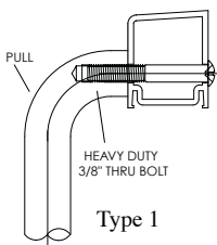
Type 1 Thru Bolt Mount
